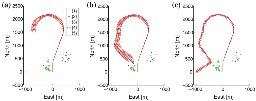
Fig. 3 A mobile robot starts from the configuration a and has to plan a motion strategy to reach a goal position, while reducing estimation uncertainty. Legend: {1} unknown environment \mathcal{W} ; {2} Goal; {3–4} Actual and estimated trajectories of the robot with 1\sigma uncertainty bounds; {5} mapped environment \mathcal{W}_k . a Robot trajectory before planning begins. b Trajectory before loop closure. Planned motion (for L = 5 look ahead steps) is shown by diamond marks. c Final trajectory after reaching the goal
