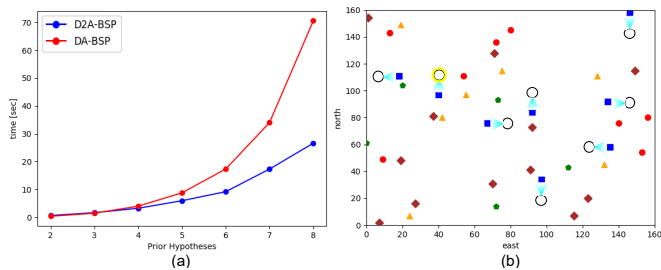
Fig. 1: Given a multi-modal initial belief, the agent’s goal is to fully disambiguate between all hypotheses. (a) Run-time [sec] as a function of number of prior hypotheses M_0 ; (b) A scenario with 8 prior hypotheses, each initialized in front of a blue square and denoted by a black ellipse. Headings are denoted with cyan triangles. The component that corresponds to the correct data association hypothesis, unknown to the agent, is highlighted in yellow.
