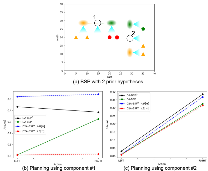
Fig. 2: (a) A scenario under hard budget constraints of Q = 6 . The agent can only move LEFT or RIGHT. Black ellipses and cyan triangles denote prior hypotheses and headings, respectively. Each prior weight equals \frac{1}{2} . Green and Orange ellipses denote the propagated belief after moving left or right, respectively. Moving LEFT is the best action as it is the only action that might lead to full disambiguation; (b) Objective function evaluations considering only component 1 (denoted by superscript Q ). DA-BSP in green represents the solution with no budget constraints considering all hypotheses; (c) Objective function evaluations considering only component 2. Notations remain the same.
